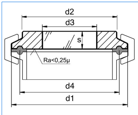
Typical assembly
