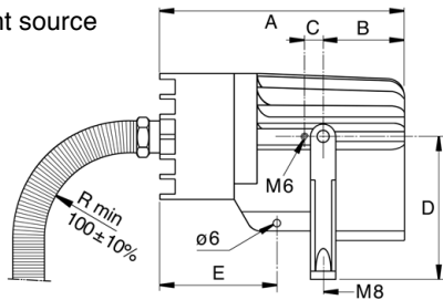
Light source
